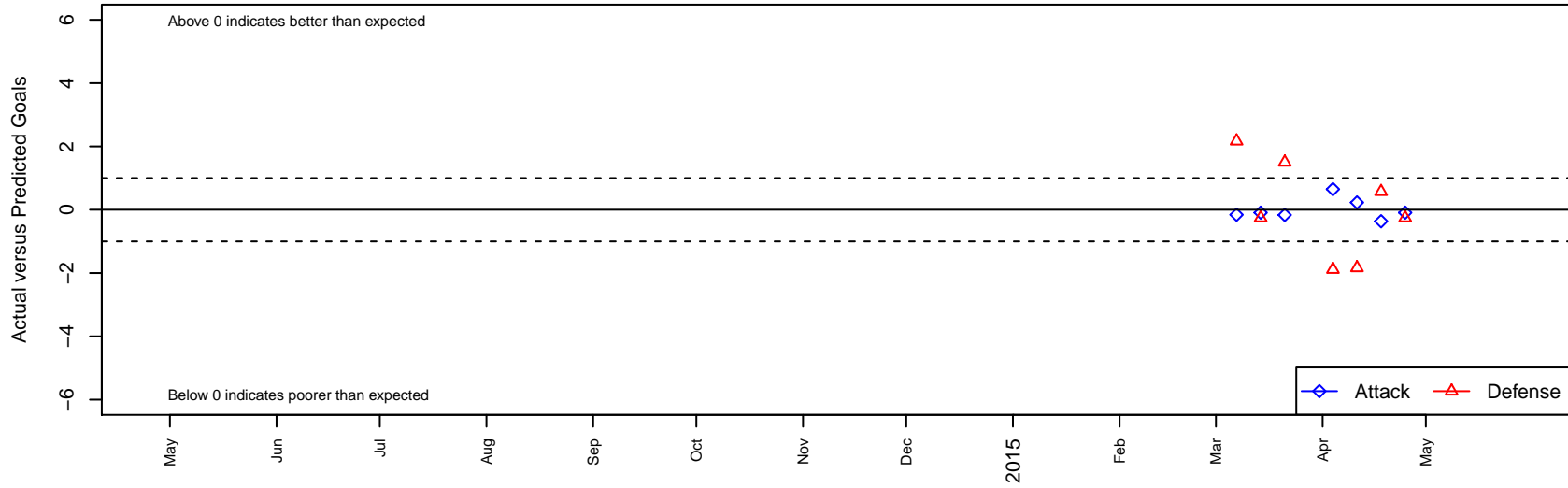
Mountain Home SC B96 Dots are actual minus expected GF (blue circles) and GA (red triangles). Blue line is smoothed change in attack strength. Red is smoothed change in defense strength.
